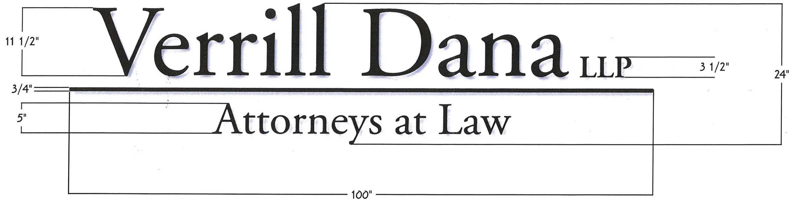
① Front Elevation Not To Scale
